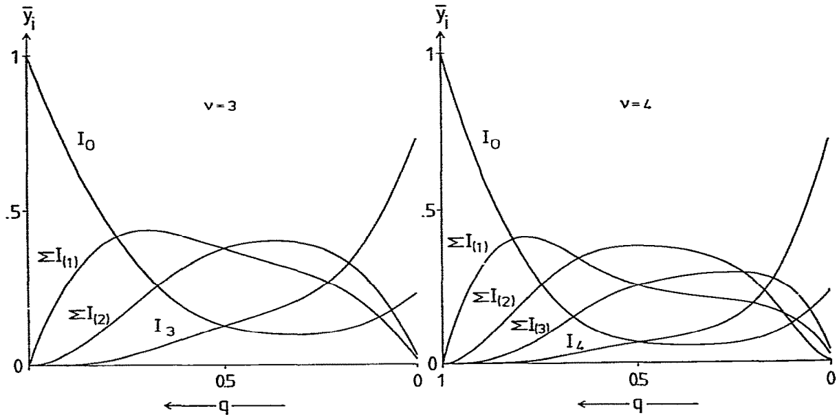
Fig. 7. Distribution of mutant classes as a function of single-digit accuracy q ( v=3 and 4). By \Sigma I_{(m)} we denote the sum of all m -error mutants of the master sequence I_0 . These are all mutants which are characterized by a Hamming distance D=m from the master sequence. The corresponding sum of concentrations is denoted by \bar{y}_m . At the point of stochastic replication ( q=0.5 ) all sequences are present in equal amounts. The distribution of mutant classes then is given by the binomial coefficients: \bar{y}_m = \binom{v}{m} \cdot 2^{-v} . Numerical values chosen are the same as in fig. 6 ( A_0=10 ; A_i=1 , i=0 , all D_i equal).
